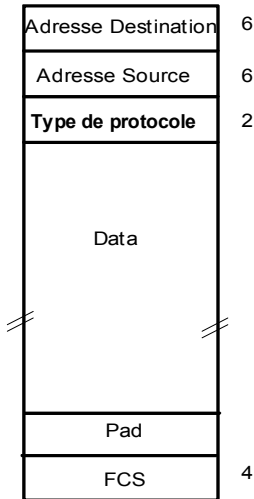
Ethernet II
