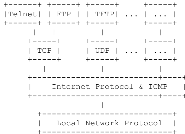
Protocol Relationships
