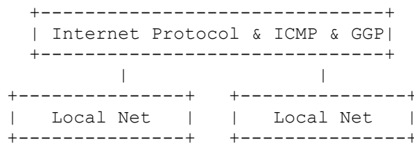
Gateway Protocols
